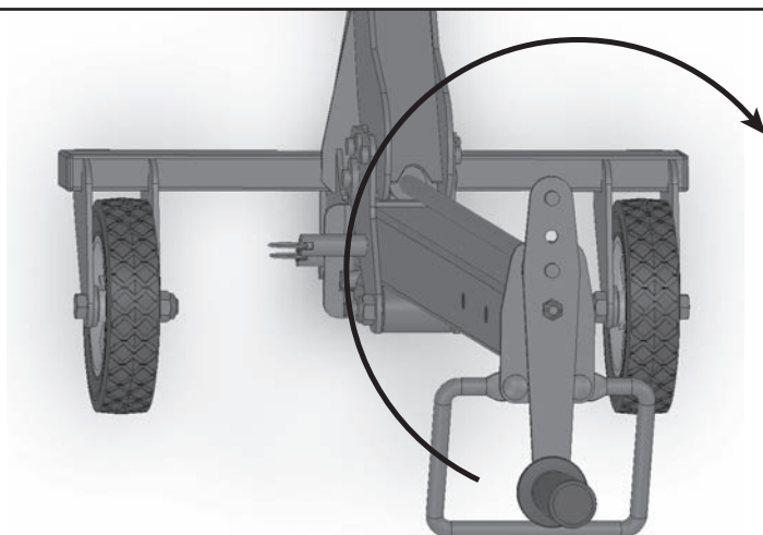
Shorter Setting – 6" Radius
