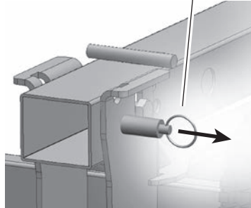
Crossbar in channel Tower Locking Pin (locked position)
